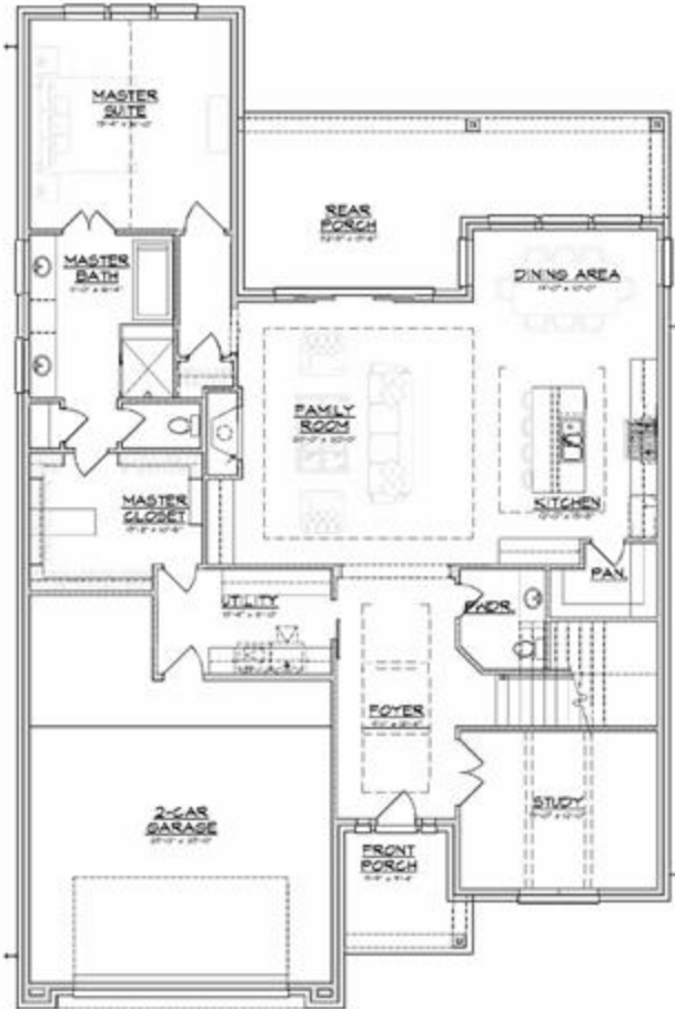
FIRST FLOOR PLAN ALL AREAS 47'x100'
